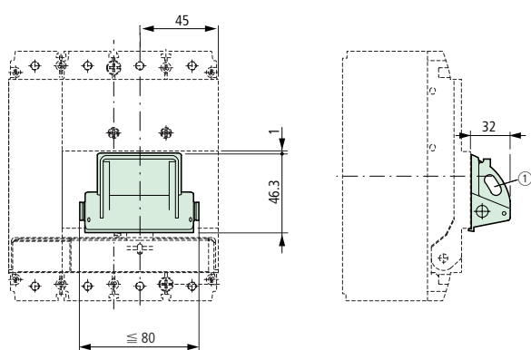
Toggle lever interlock device NZM1-XKAV
