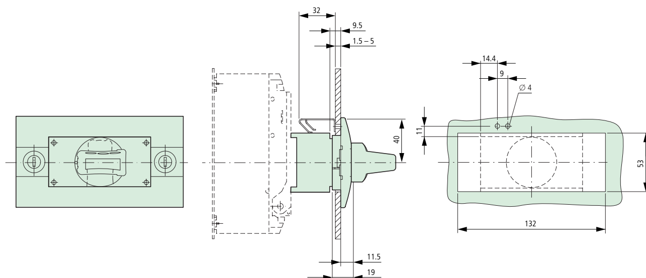
Rotary handle on switch with door interlock NZM1-XDTV(R)
